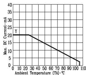
Fig5. MAX. ALLOWABLE DC CURRENT VS. AMBIENT TEMPERATURE.
