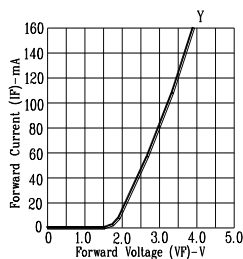
Fig3. FORWARD CURRENT VS. FORWARD VOLTAGE
