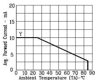
Fig8. MAX. AVERAGE FORWARD CURRENT VS. AMBIENT TEMPERATURE.
