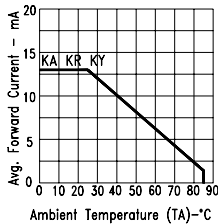
Fig.4. Max. Average Forward Current vs. Ambient Temperature.
