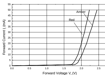
Fig.2 Forward voltage vs. forward current
