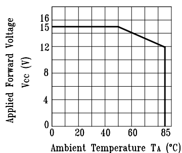
Fig.4. Maximum Allowed Applied Forward Voltage vs. 12 Volts Devices
