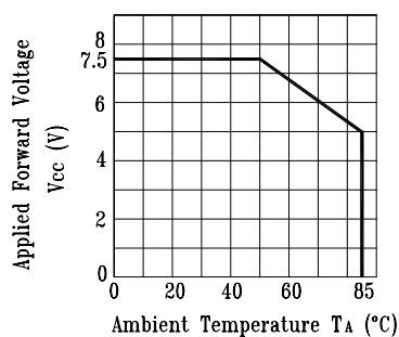
Fig.4. Maximum Allowed Applied Forward Voltage vs. 5 Volts Devices
