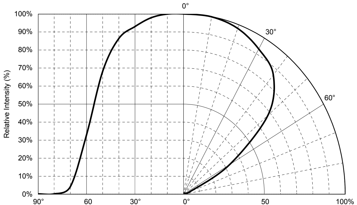
Fig 2. Radiation Characteristics
