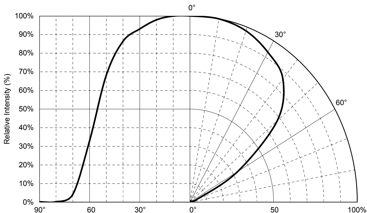
Fig 2. Radiation Characteristics
