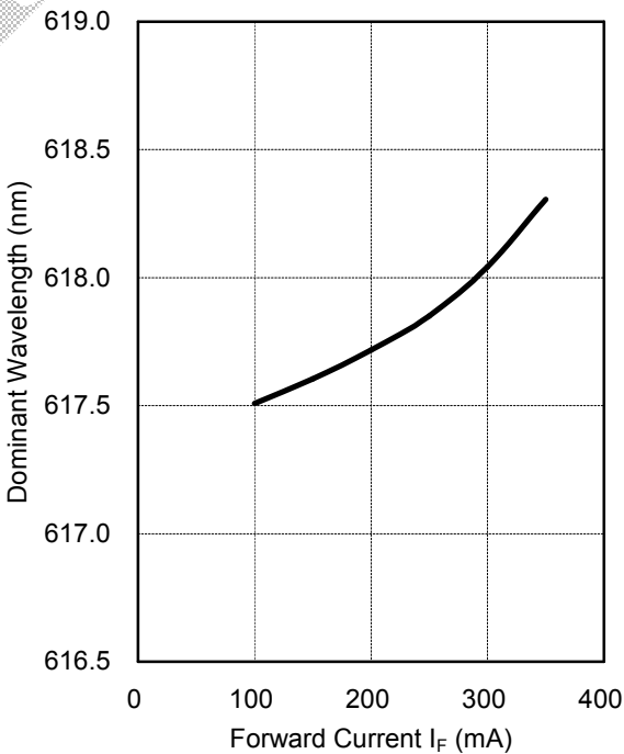
Fig 5. Wavelength Shift
