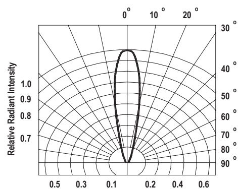
Figure 6. Radiation Diagram
