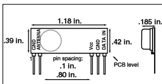
Physical Outline
