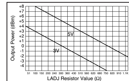
Figure 7: Output Power vs. LADJ Resistor
