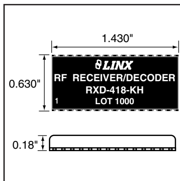
Figure 1: Package Dimensions
