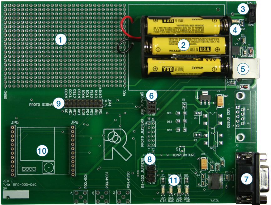
Figure 3: 250 Series Transceiver Development Board
