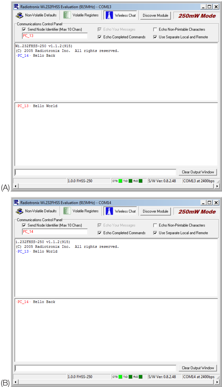
Figure 13: 250 Series Development System Software Wireless Chat Tab; Response (A) Received; (B) Sent
