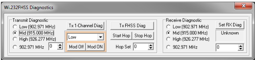
Figure 20: 250 Series Transceiver Development System Software Diagnostics Window
