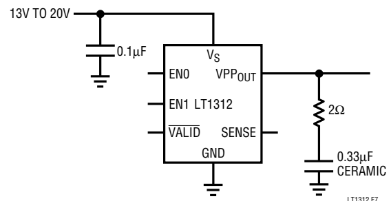
Figure 7. Using a 0.33 \mu F to 1 \mu F Output Capacitor
