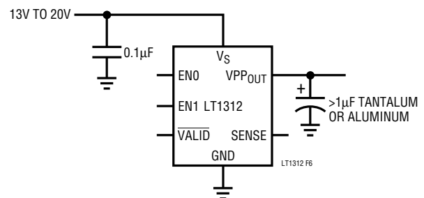
Figure 6. Recommended >1 \mu F Tantalum Output Capacitor
