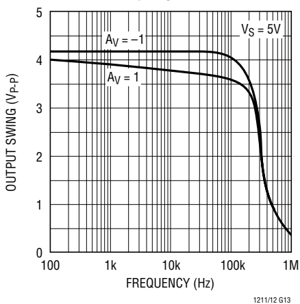
Undistorted Output Swing vs Frequency, V_S = 5\text{V}
