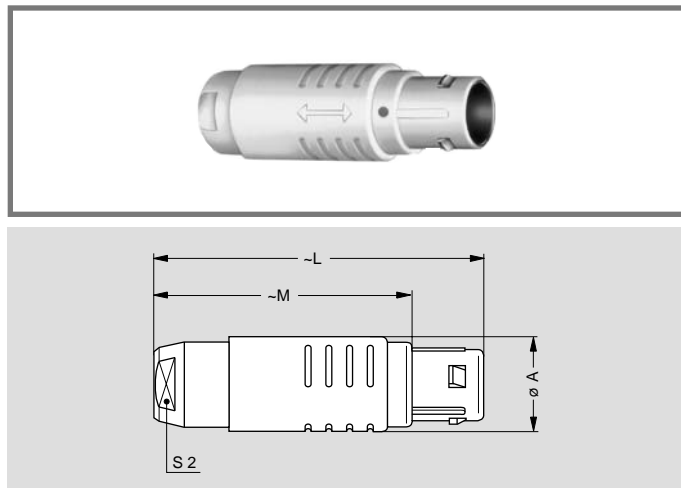
FGY Straight plug, keys (Y), cable collet and PSU or PPSU outer shell
