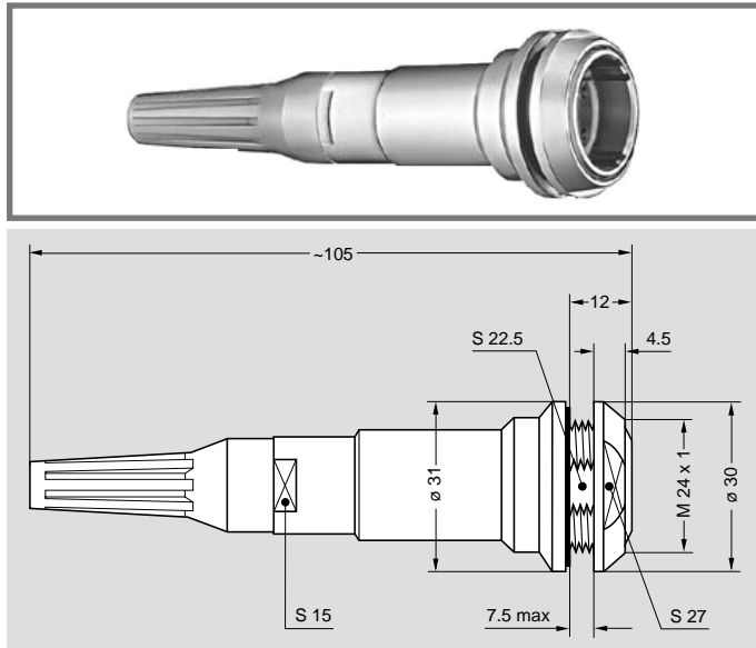
PEW.3K Fixed receptacle, nut fixing, keys (W), cable adapter, with bend relief (back panel mounting)
