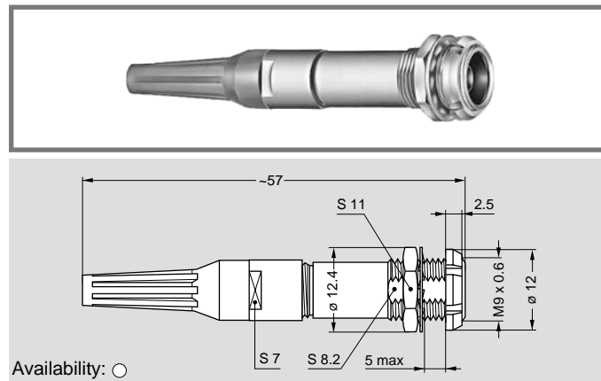
PFG.0B Fixed receptacle, with two nuts, key (G) or keys (A...F), with bend relief, (back panel mounting)
