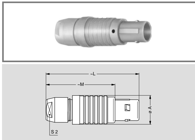
FGG Straight plug, key (G or J), cable collet, PEEK outer shell
