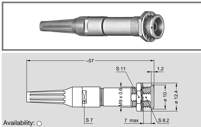
PKG.0B Fixed receptacle, nut fixing, key (G) or keys (A...F), with bend relief
