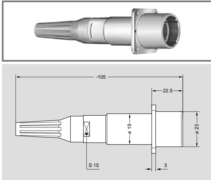
PBW.3K Fixed receptacle with rear square flange (4 holes fixing), keys (W), cable adapter, with bend relief
