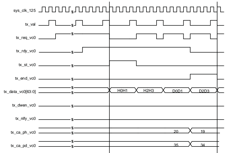
Figure 2.10. Transmit Interface 2.5G IP Core Downgraded x1 or 5G IP core Downgraded x1 at Gen1 speed
