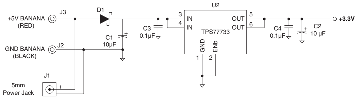
Figure 3. On-Board Power Supply
