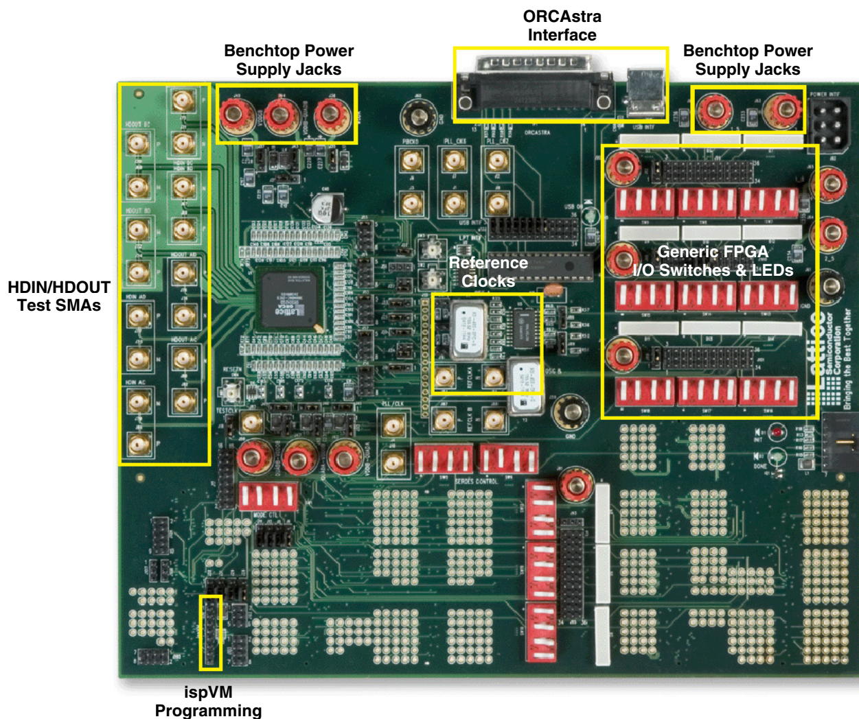
Figure 1. ORT/ORSO42G5 High-Speed SERDES Board
