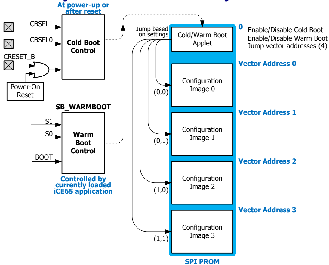
Figure 27: ColdBoot and WarmBoot Configuration
