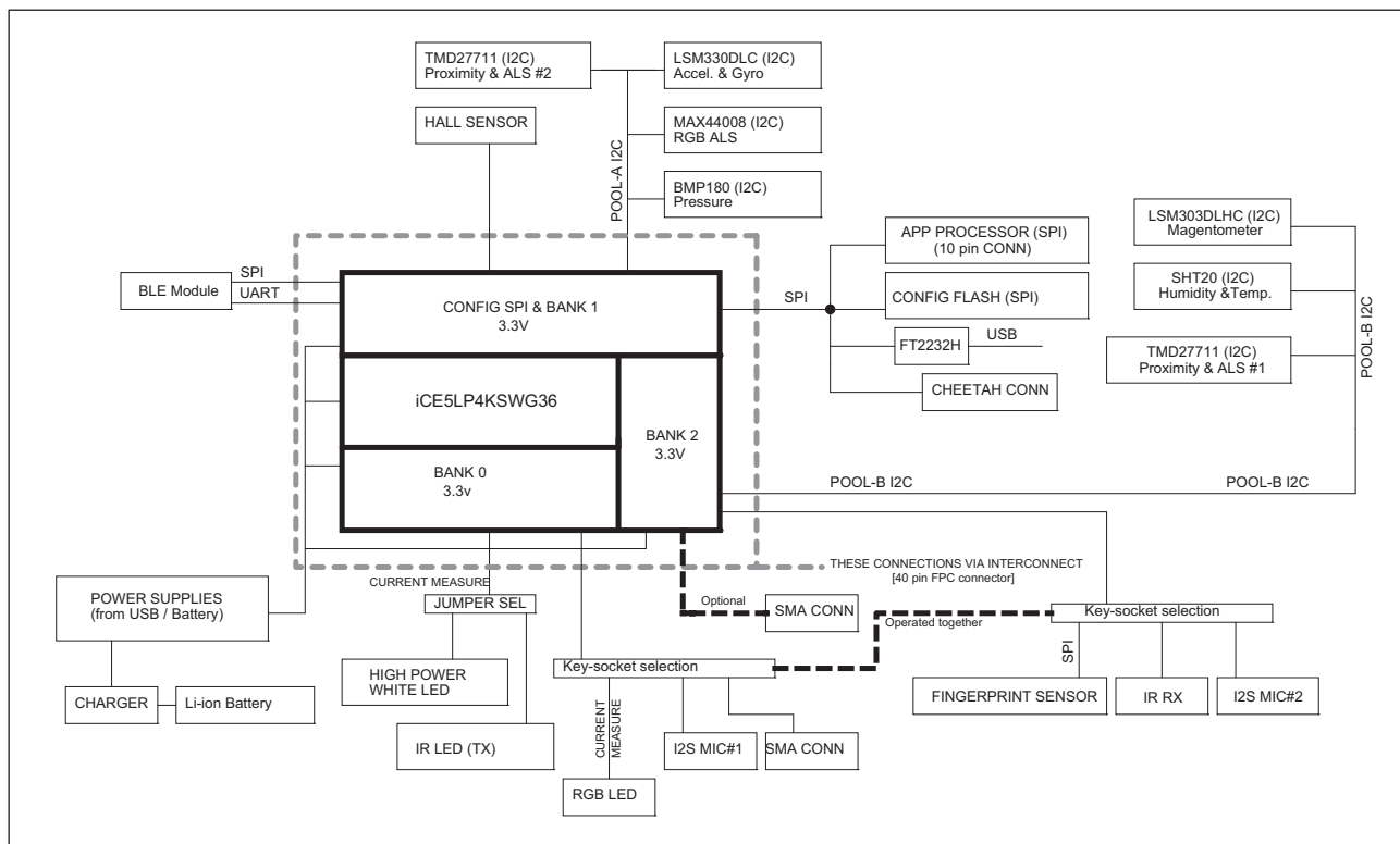
Figure 1. Block Diagram
