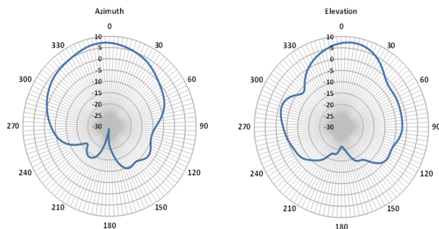
Radiation Pattern at 2412 MHz
