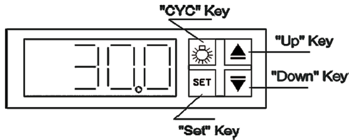
Figure 3 - User Interface
