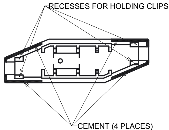
CEMENT AND AL CLIP POSITIONS INSIDE OF MICBOX CASE
