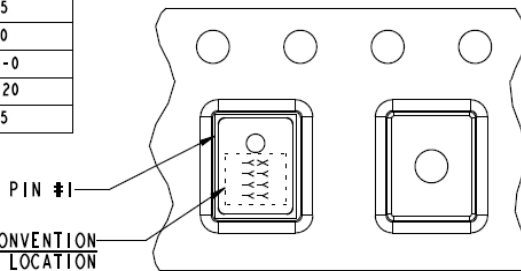
COMPONENT ORIENTATION
