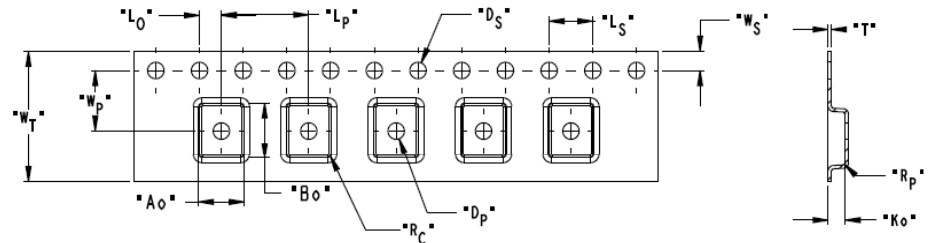
COMPONENT ORIENTATION
