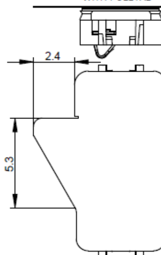
RECEIVER WITH PULL TAB
