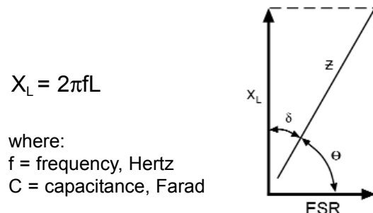
Figure 4b: Total Impedance of the Capacitor Above Resonance
