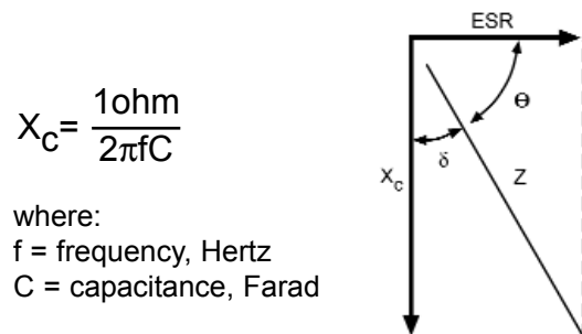
Figure 4a: Total Impedance of the Capacitor Below Resonance
