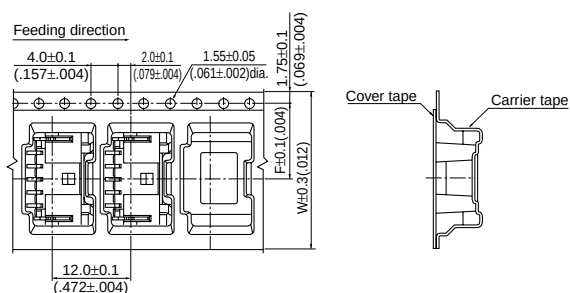
Side entry type (2 to 5 circuits)
