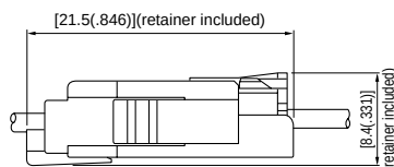
PA Receptacle + PAL Receptacle (Standard type)
