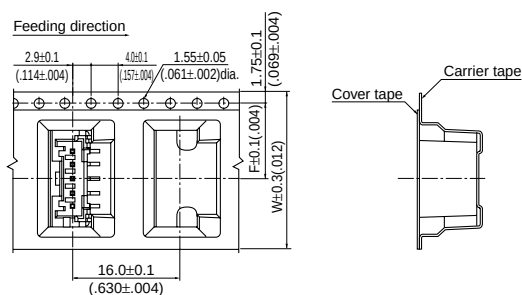
Side entry type (2 to 5 circuits)
