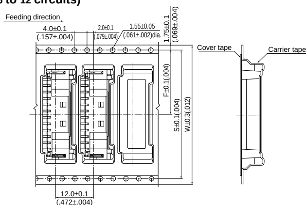
(6 to 12 circuits)
