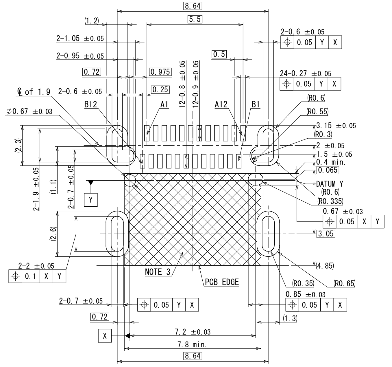
CONNECTOR MOUNTING SURFACE SIDE VIEW
