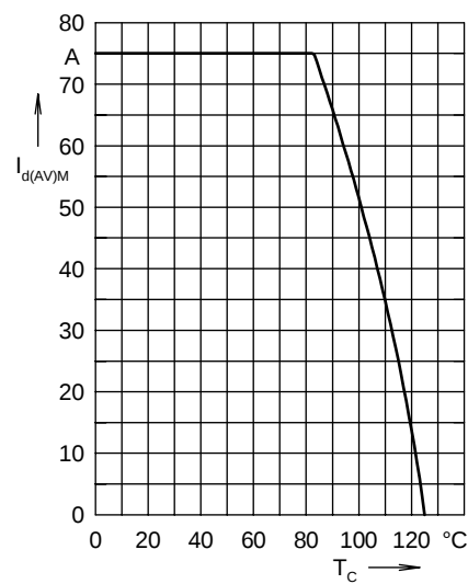
Fig. 8 Max. forward current versus case temperature
