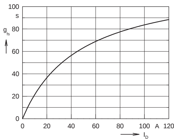
Fig. 11 Typical transconductance g_{is} = f(I_D)
