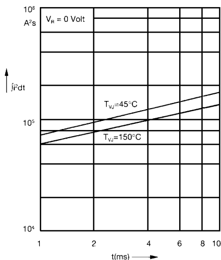
Fig. 2 \int j^2 P dt versus time (1-10 ms)
