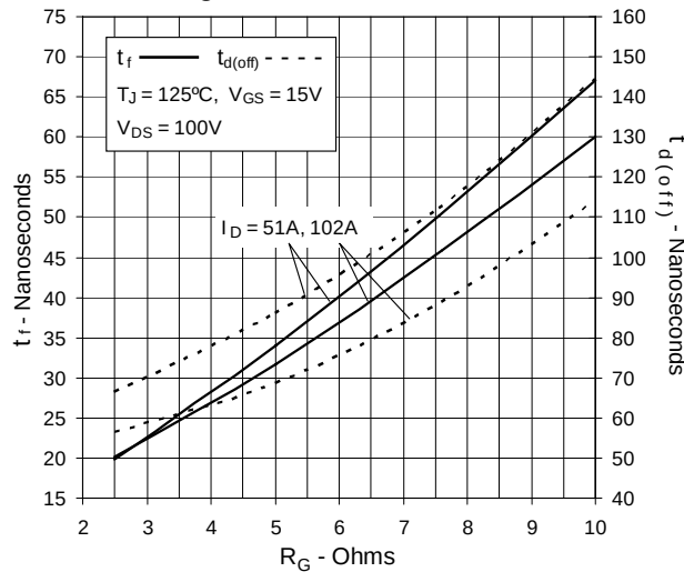
Fig. 18. Resistive Turn-off Switching Times vs. Gate Resistance
