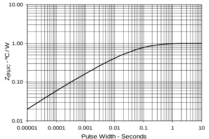
Fig. 12. Maximum Transient Thermal Resistance
