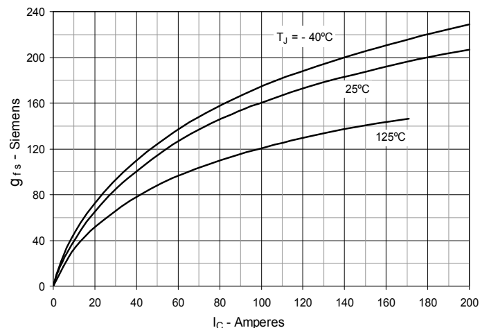
Fig. 6. Transconductance
