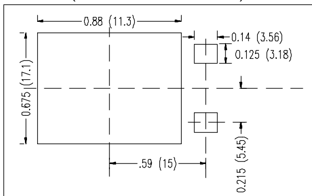
Min. Recommended Footprint (Dimensions in inches and mm)
