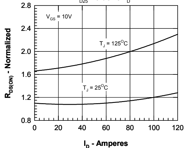
Figure 3. R_{DS(on)} normalized to 0.5 value vs. I_D
