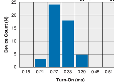
TS190L Typical Turn-On Time (N=50 Ambient Temperature = 25°C) (Load Current = 150mA DC ; I_F = 5\text{mA}_{DC} )
