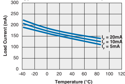
TS190L Typical Load Current vs. Temperature
