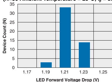
TS190L Typical LED Forward Voltage Drop (N=50 Ambient Temperature = 25°C; I_F = 5\text{mA}_{DC} )
