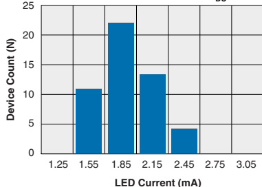
TS190L Typical I_F for Switch Operation (N=50 Ambient Temperature = 25°C) (Load Current = 150mA DC )
