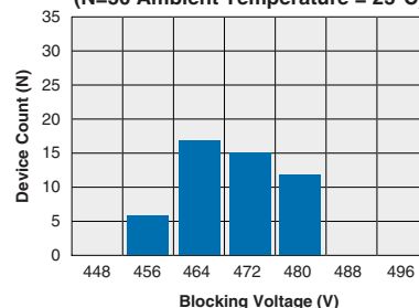
TS190L Typical Blocking Voltage Distribution (N=50 Ambient Temperature = 25°C)
