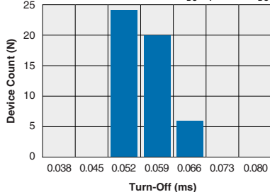
TS190L Typical Turn-Off Time (N=50 Ambient Temperature = 25°C) (Load Current = 150mA DC ; I_F = 5\text{mA}_{DC} )
