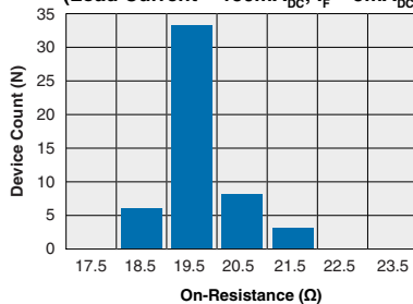
TS190L Typical On-Resistance Distribution (N=50 Ambient Temperature = 25°C) (Load Current = 150mA DC ; I_F = 5\text{mA}_{DC} )
