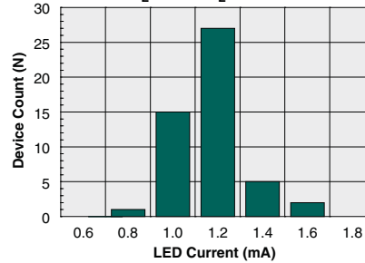
Typical I_F for Switch Operation Resistive Load (N=50, I_L=1.5\text{A} , V_L=120\text{VAC}/60\text{Hz} )
