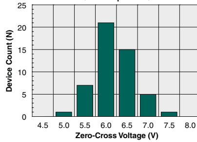
First Zero-Cross Turn-On Voltage Distribution (N=50, I_F=5\text{mA} )
