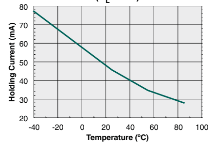
Holding Current vs. Temperature ( R_L=1.9\Omega )
