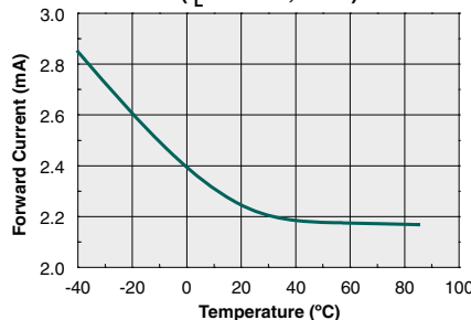
LED Forward Current to Operate vs. Temperature - Resistive Load ( I_L=350\text{mA} , 60Hz)
