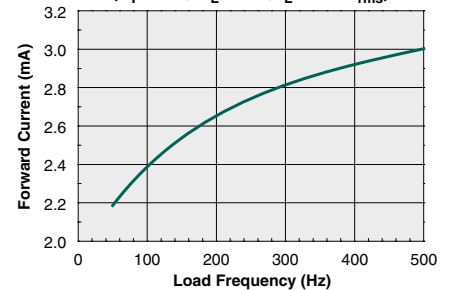
LED Forward Current to Operate vs. Load Frequency ( V_P=67\text{V} , R_L=50\Omega , I_L=0.94\text{A}_{\text{rms}} )
