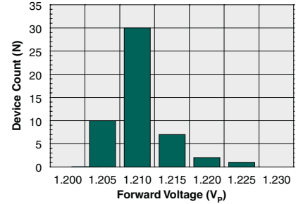
On-State Forward Voltage Drop (N=50, I_F=5\text{mA} , I_L=1.5\text{A} )
