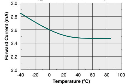
LED Forward Current to Operate vs. Temperature - Inductive Load ( I_L=500\text{mA} , 60Hz, 200mH)
