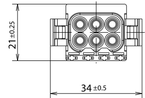
Plug, 6 poles
