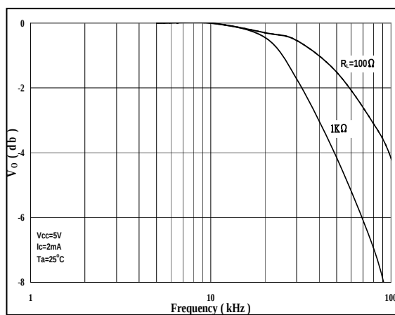
Fig 11 Frequency Response
