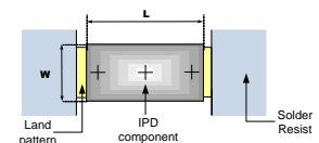
(1206 PCB footprint)
