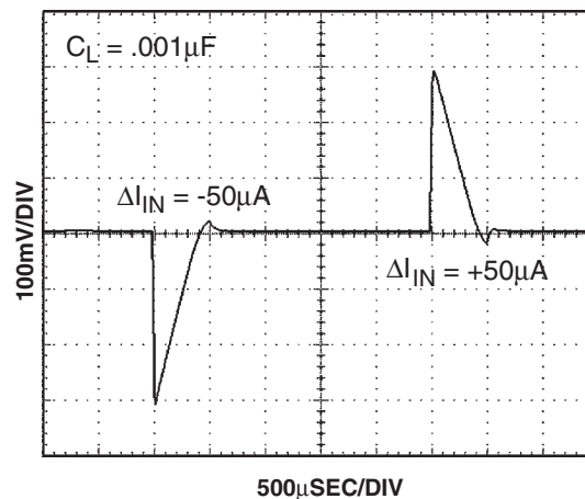
50μA LOAD TRANSIENT RESPONSE
