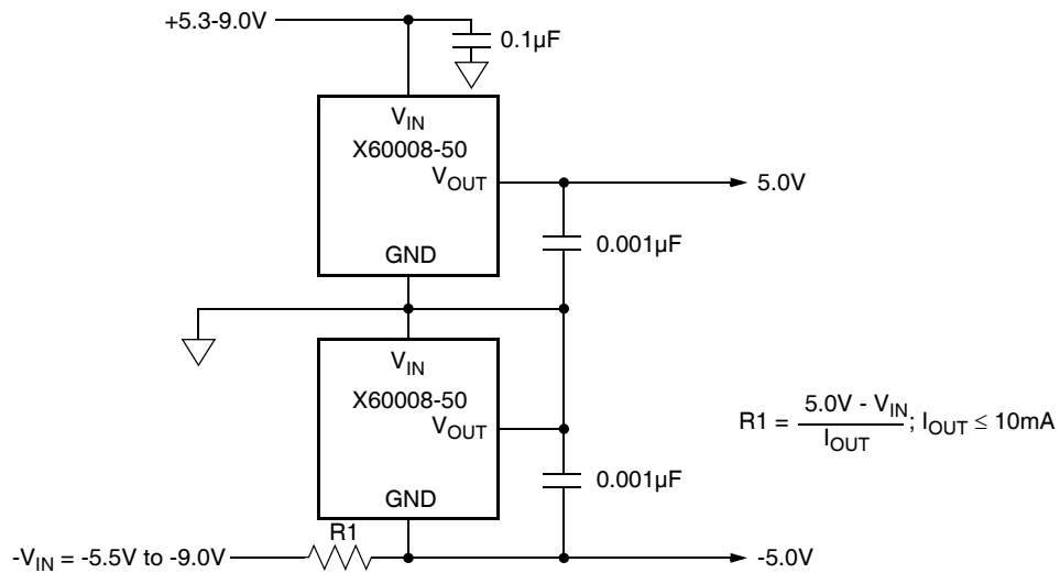
\pm 5.0V Dual Output, High Accuracy Reference
