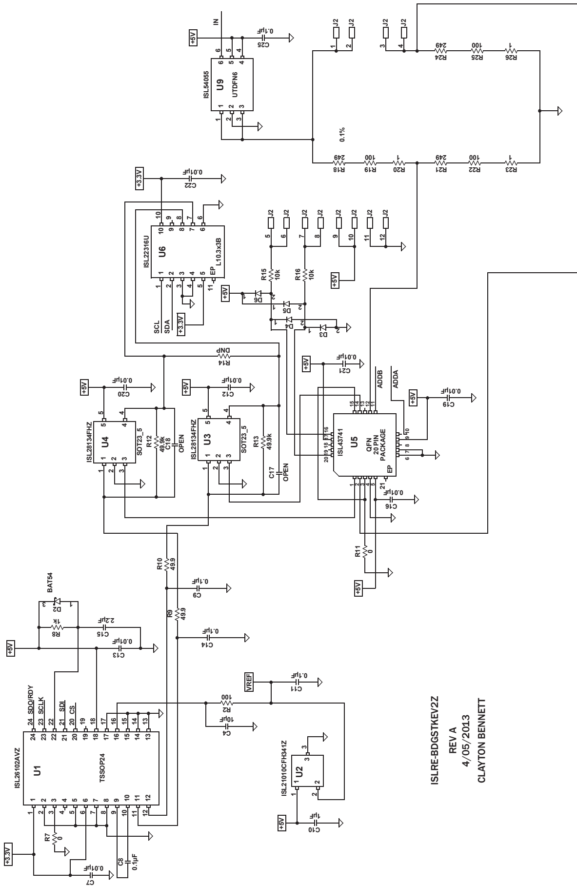
FIGURE 10. ISLRE-BDGTKEV2Z STRAIN GAUGE SCHEMATIC
