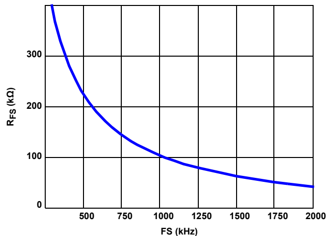
FIGURE 62. R_{FS} SELECTION vs F_S
