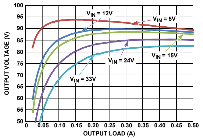
FIGURE 20. EFFICIENCY vs LOAD, PWM, V_{OUT} = 3.3\text{V}
