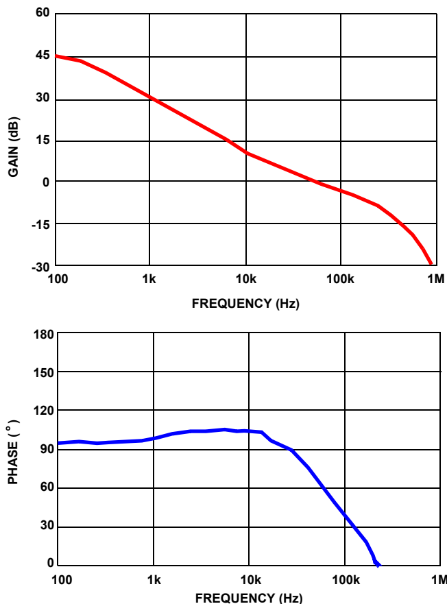
FIGURE 65. SIMULATED LOOP GAIN
