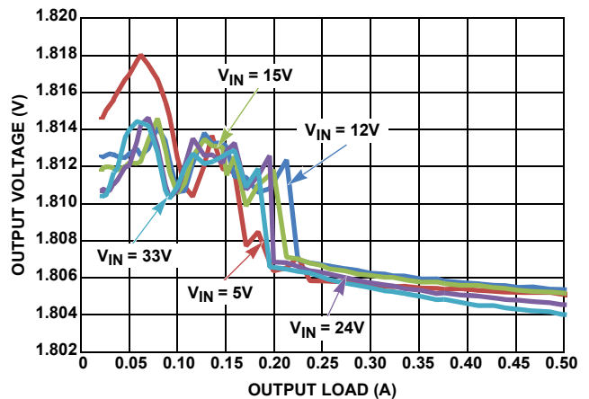
FIGURE 31. V_{OUT} REGULATION vs LOAD, PFM, V_{OUT} = 1.8\text{V}
