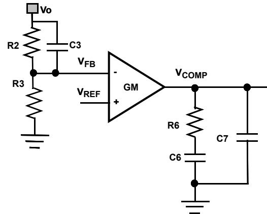
FIGURE 64. TYPE II COMPENSATOR
