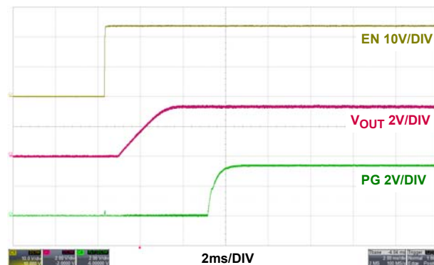
FIGURE 57. POWER-GOOD DELAY, PWM ( I_{OUT} = 0A )
