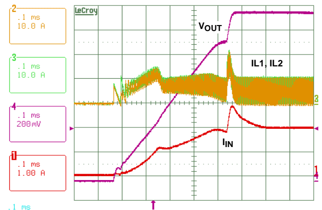
FIGURE 13. INRUSH CURRENT AT START-UP, V_{IN} = 8V, VID = 1.4375V, I_{LOAD} = 10A
