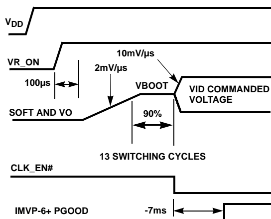
FIGURE 34. SOFT-START WAVEFORMS USING A 20nF SOFT CAPACITOR
