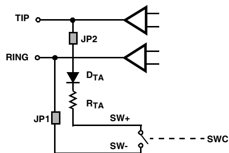
FIGURE 4. TEST LOAD SWITCHING
