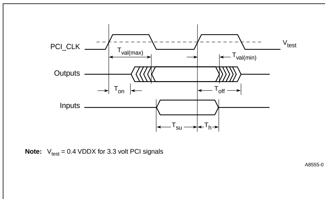
Figure 15. PCI Bus Signals
