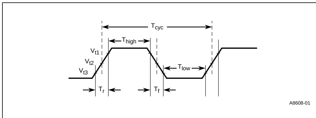
Figure 61. SRAM SCLK Signal AC Parameter Measurements
